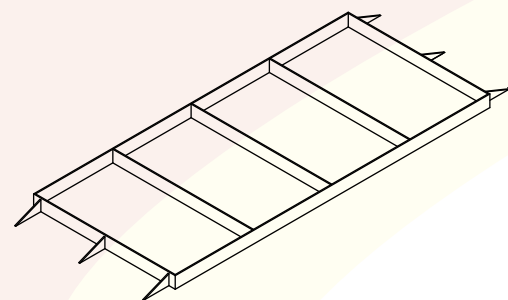
SKELETAL FRAME (TOP PLATES REMOVED)
